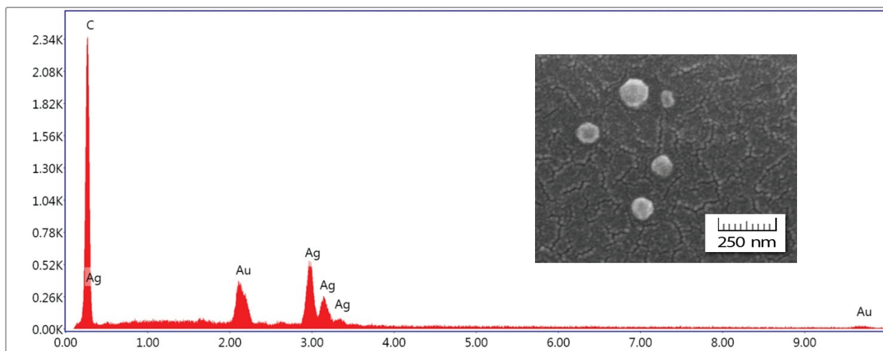
Figure 2 EDX pattern of silver nanoparticles prepared by ascorbic acid as reducing agent (AA 35)
