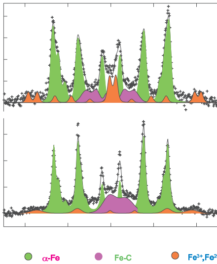
Fig. 4 Mössbauer spectra of the brake disc taken in scattering geometry with detection of 14.4 keV gamma radiation (top) and with detection of conversion electrons (bottom)
