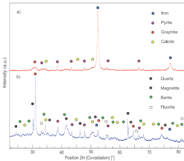
Fig. 2 Top: XRD pattern of the powder sample prepared by ball milling of the brake pad and brake disc materials for 14 hrs. Bottom: XRD pattern of the powder sample obtained by sweeping of the surface of brake pads and brake disc
