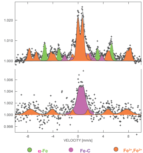
Fig. 5 Mössbauer spectra of the brake pad taken in scattering geometry with detection of 14.4 keV gamma radiation (top) and with detection of conversion electrons (bottom)
