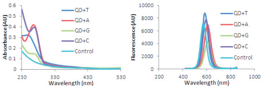
Fig. 2 Absorbance and fluorescence of QDs. CdTe/ZnSe QDs conjugated with T, A, G and C are represented as QD+T, QD+A, QD+G and QD+C respectively. Utilized excitation wavelength was 380 nm within all cases
