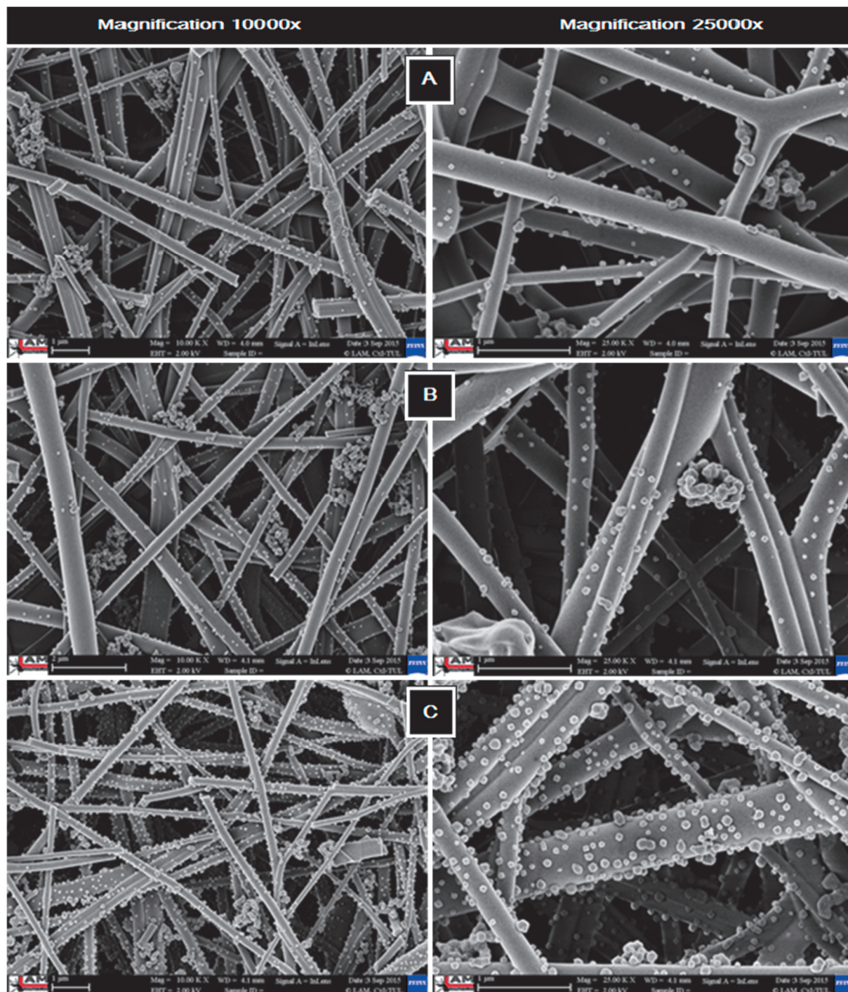
Fig. 2 SEM images of silica/PVA nanofibers with immobilized Ag ions in different magnifications.
