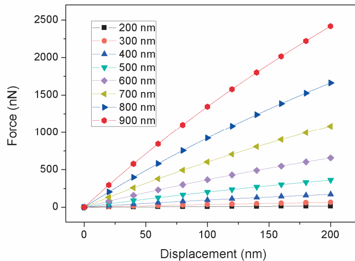
Fig. 5 The force-distance simulation where the outer diameter of CNT is a parameter. The length of CNTs is 50 \mu\text{m} . The Young's modulus of CNT is set to be of 500 GPa. The interaction is assumed to be with one CNT in contact at once as it was in all previous cases.
