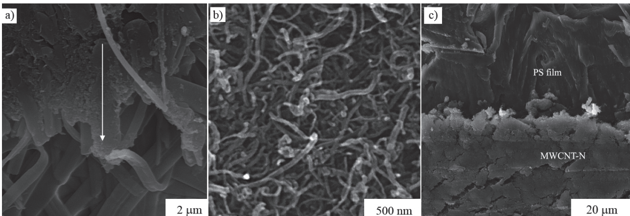
Fig. 2 Part a) SEM analyses of profile view of cut thought PS filter/MWCNT structure where arrow indicates filtration direction. Part b) SEM image of the surface of entangled MWCNT network. Part c) SEM analyses demonstrating the transformation of PS non-woven filtrating membrane into form of PS thin film with interlocked carbon nanotubes network.
