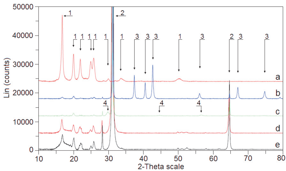
Fig. 2 XRD pattern of prepared samples PP (a), PP/GRA2Zn (b), PP/GRA1Ti (c), PP/GRA2 (d), and PP/GRA1 (e) before thermal treatment. 1 - \alpha -polypropylene, 2 - graphite, 3 - ZnO, 4 - TiO 2
