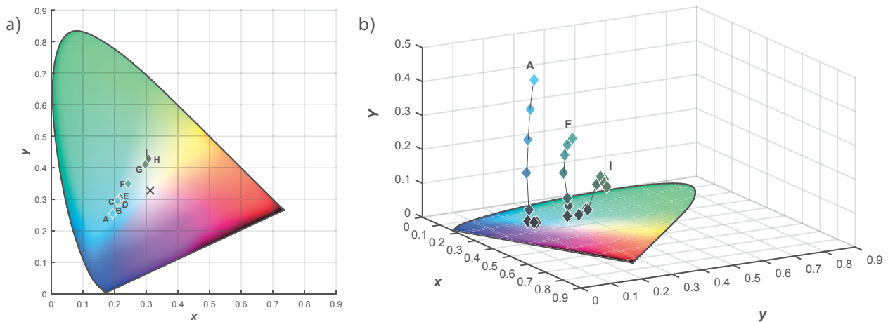
Fig. 5 CIExyY colorimetric model showing a) trichromatic positions of all samples after 144 hours of stirring and b) colour changes in time of samples A, F and I where the start of the synthesis process is at the lowest values of Y; for a clearer view, the volume of CIExyY space for Y > 0 was not rendered
