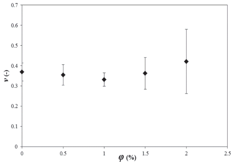
Fig. 5 Poisson's ratio ( \nu ) of Epoxy nanocomposites with different weight fractions ( \phi ) of CNTs
