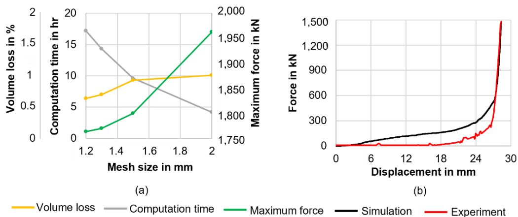
Figure 5 (a) Mesh sensitivity study and (b) comparison of simulated and experimental force-displacement curves
