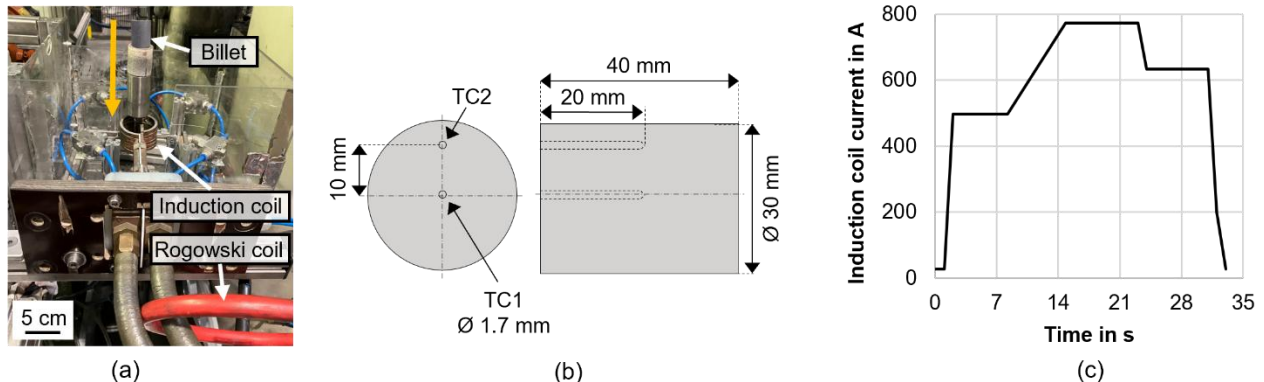
Figure 2 (a) Experimental setup of induction heating, with billet movement indicated by the yellow arrow, (b) TC positions in the billet, and (c) measured current in the induction coil using a Rogowski coil
