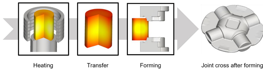
Figure 1 Process chain consisting of induction heating, billet transfer and single-stage closed-die forging
