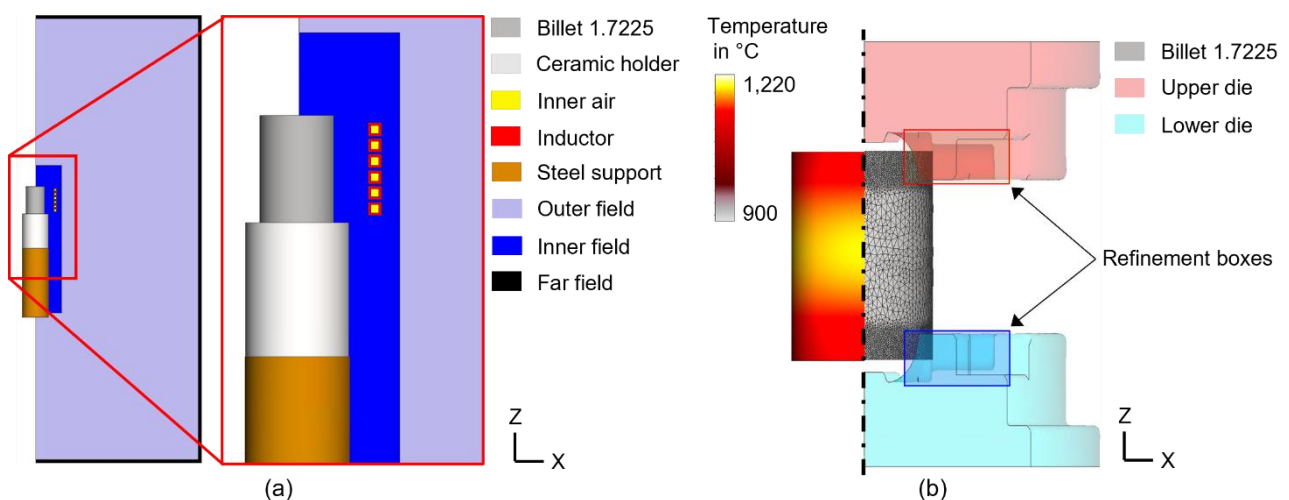
Figure 3 Simulation model of (a) induction heating [4], and (b) closed-die forging
