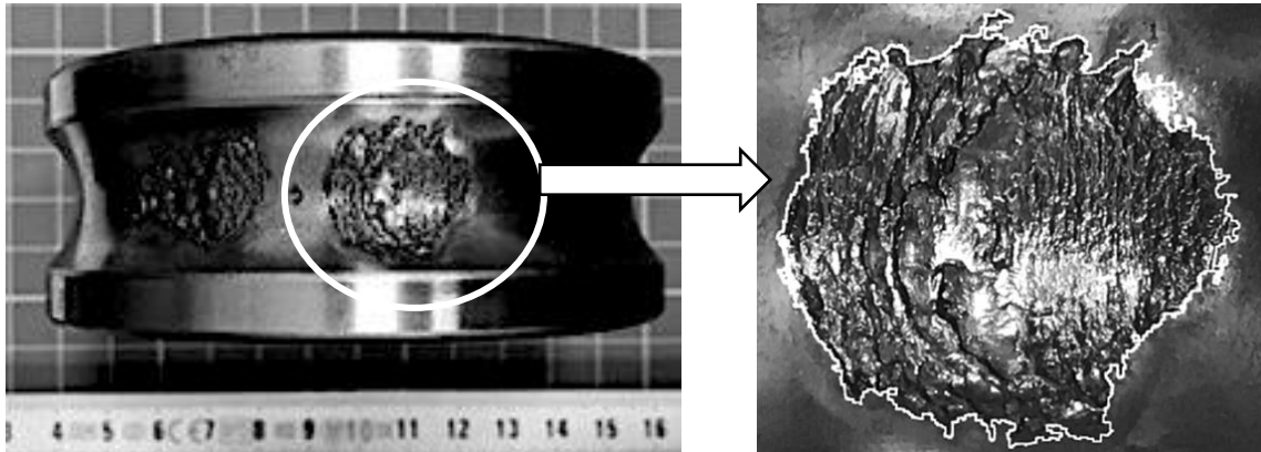
Figure 3 Digital image analysis of fatigue changes of the inner raceway of a rolling bearing
