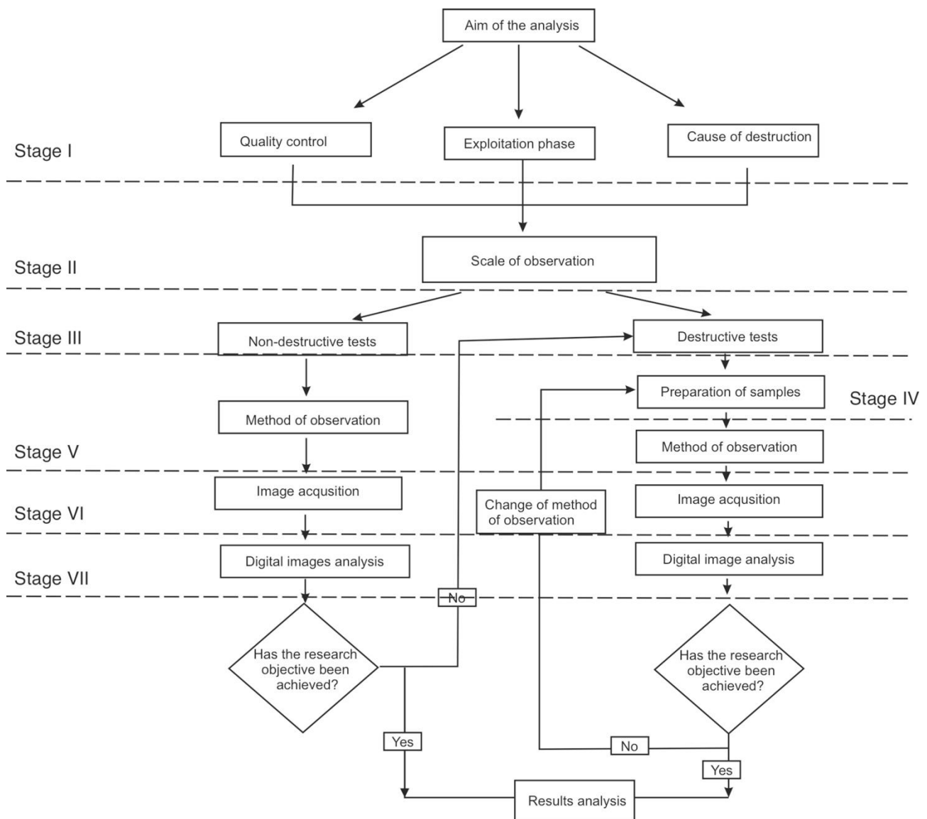
Figure 1 Model of the process identification of the material structures
