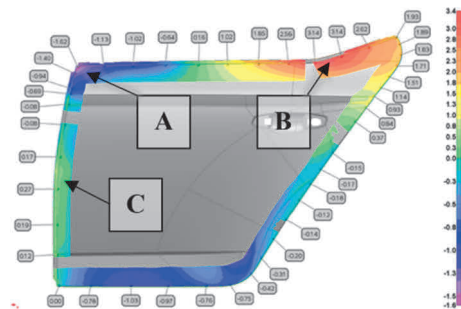
Figure 5 Springback measurement result, DP500
