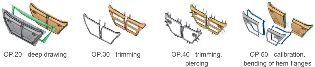
Figure 2 ŠKODA FABIA, CAD data of tools
