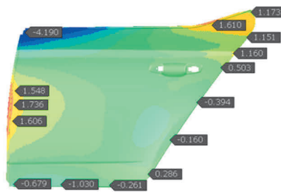
Figure 7 Springback in normal direction, DP500, MTC 2
