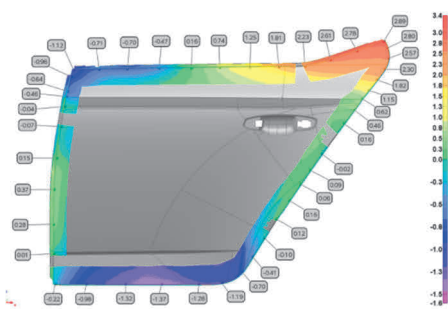
Figure 4 Springback measurement result, HX180BD
