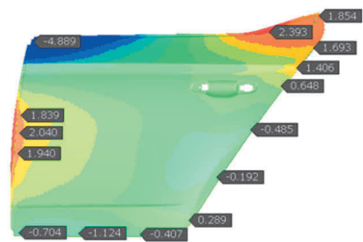
Figure 8 Springback in normal direction, DP500, MTC 3
