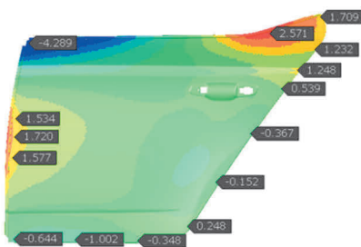
Figure 6 Springback in normal direction, DP500, MTC 1
