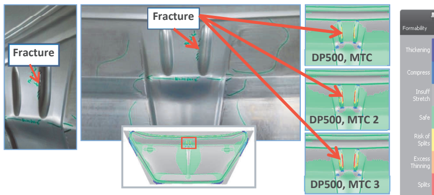
Figure 3 "Formability" after OP.20 (Deep Drawing)
