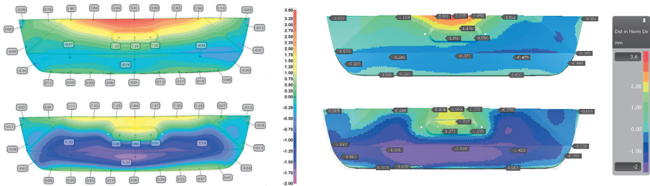
Figure 11 Left: Virtual springback in normal direction, DC05 (above) and DP500 - MTC 1 (below); right: Virtual springback in normal direction, DC05 (above) and DP500 - MTC 1 (below)
