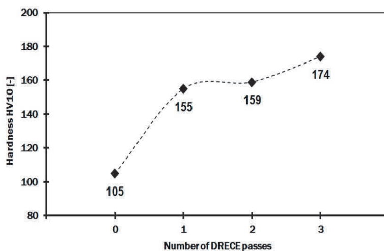
Figure 4 Vickers hardness HV_{10} evolution during DRECE processing
