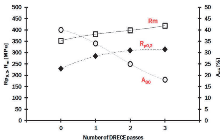
Figure 5 Tensile properties of CuZn37 with dependence of number of DRECE passes
