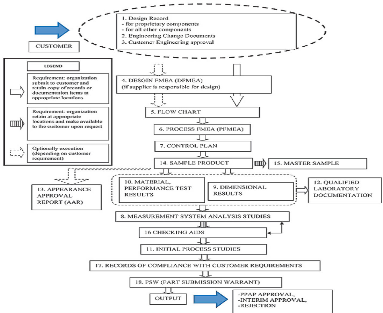
Fig. 1 The flow chart of preparing PPAP documentation at level 3 [1]
