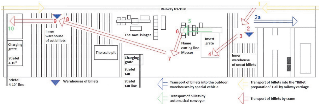
Fig. 4 Sankey diagram for transport of material in the „Billet preparation“ Hall
