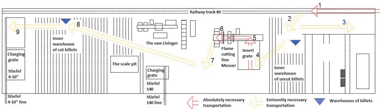
Fig. 3 Sankey diagram for determination of the distances and the necessity of material flow in the "Billet preparation" Hall
