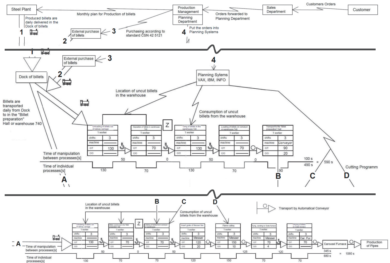
Fig. 6 Value Stream Design (VSD) in "Billet preparation" Hall
