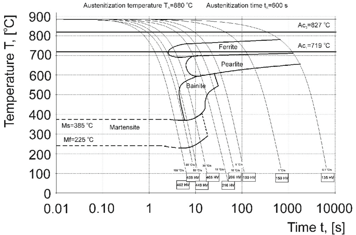
Fig. 7 Real TTT diagram for 20MnB4 steel
