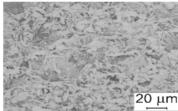
Fig. 6 Microstructure of 20MnB4 steel composed of the mixture of pearlite and ferrite cooled after deformation at the rate of 10 °C/s: longitudinal section
