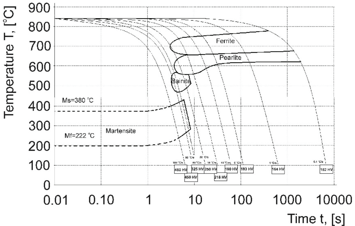
Fig. 8 Real DTTT diagram for 20MnB4 steel
