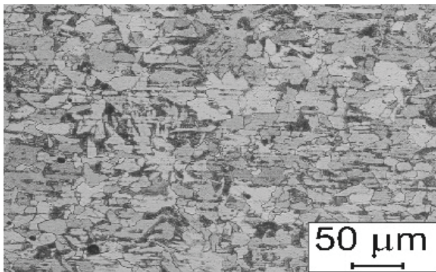
Fig. 5 Ferrite-pearlite microstructure of 20MnB4 steel cooled at the cooling rate of 1 °C/s: longitudinal section
