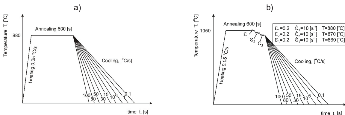
Fig. 4 Heat treatment diagrams used for preparation of TTT and DTTT diagrams for 20MnB4 steel
