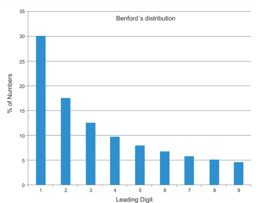
Fig. 1 Benford's Law [11]
