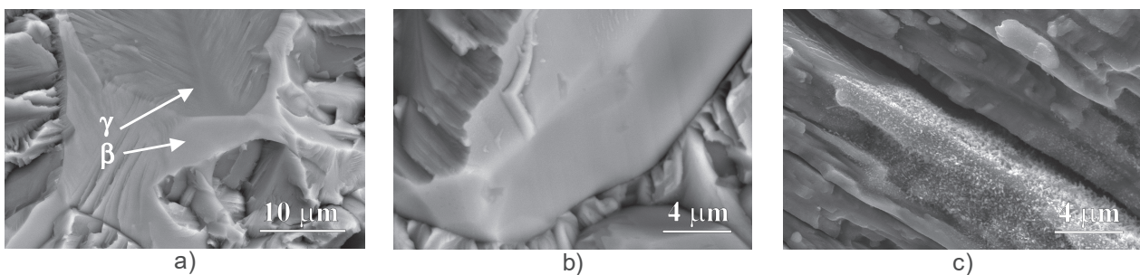
Fig. 5 a) Crack initiation site in \beta phase (brighter colour) surrounded by \gamma phase (BSE), b) inter-granular fracture caused by increased temperature (BSE), c) oxidation at 750 °C and delamination between two areas with trans-lamellar fracture with inter-lamellar secondary cracking (SE)
