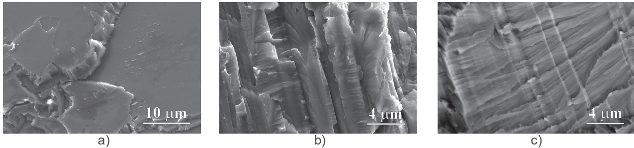
Fig. 4 a) Fracture surface with inter-lamellar fracture (SE mode), b) trans-lamellar fracture with steps corresponding to lamellae (SE), c) trans-lamellar fracture with cleavage facets and river-like ridges (BSE)
