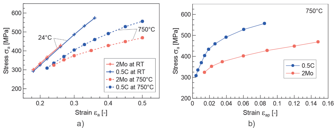
Fig. 3 a) Plot of the stress amplitude \sigma_a vs the total strain amplitude \epsilon_a for two selected alloys (2Mo and 0.5C) tested at RT and 750 °C. b) Cyclic stress-strain curves for 2Mo and 0.5C alloys tested at 750 °C
