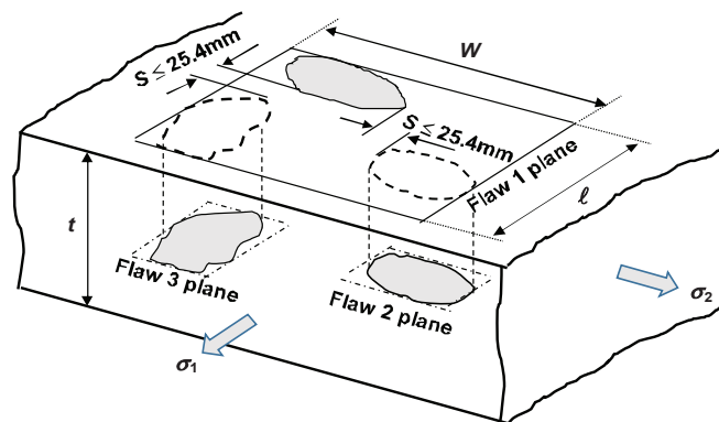
Fig. 2 Combination laminar flaws provided by the ASME Code Section XI.
