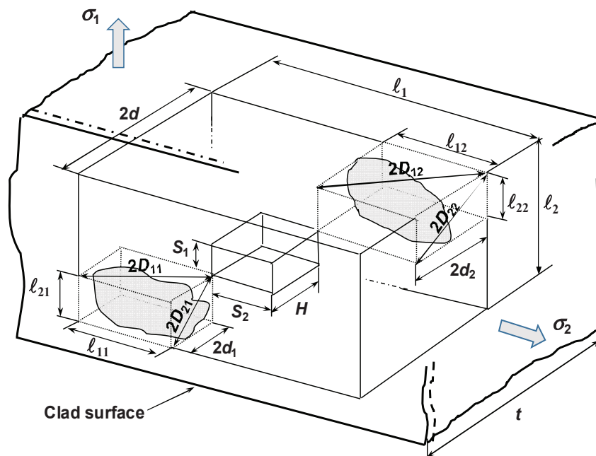
Fig. 4 nBoundig box of combined flaw for multiple quasi-laminar flaws
