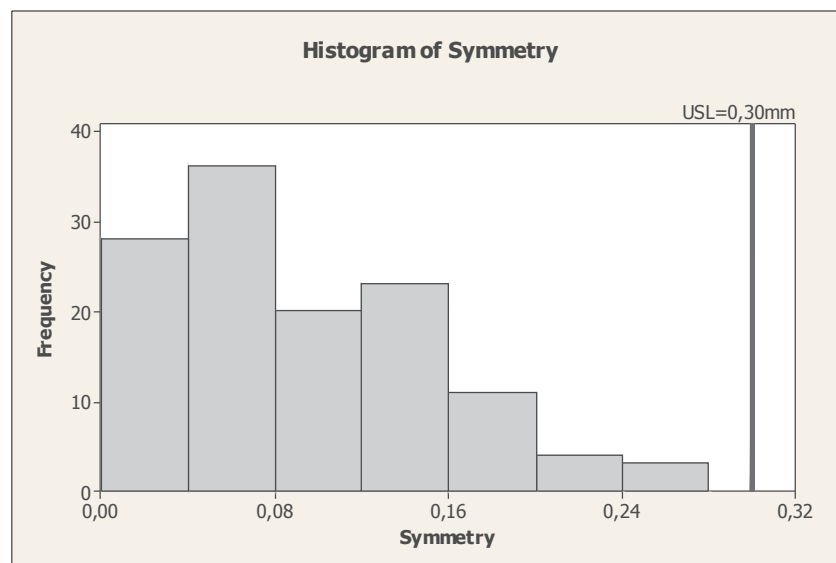
Fig. 2 Histogram of part symmetry
