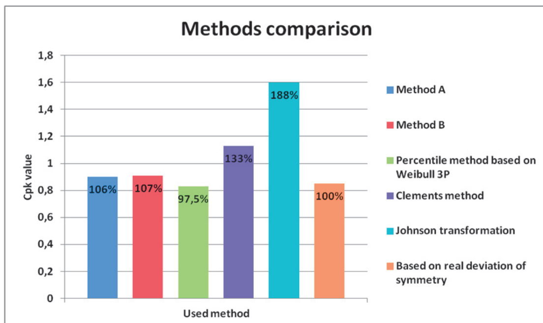
Fig. 3 Comparison of various ways of C_{pk} calculation
