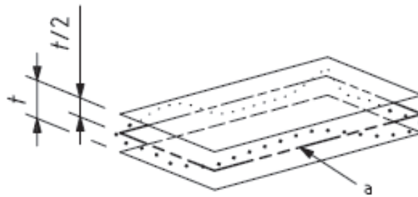
Fig. 1 Definition of symmetry tolerance zone [8]
