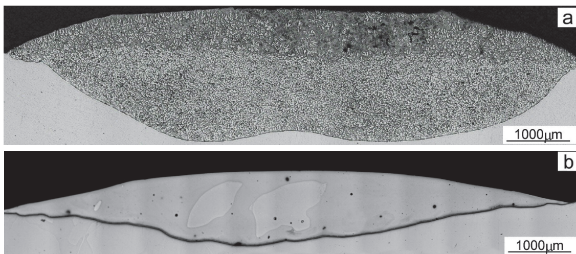
Fig. 1 Cross-sections of magnesium samples surface-alloyed with aluminum using the TIG method: (a) at a higher current (40 A), (b) at a lower current (25 A)
