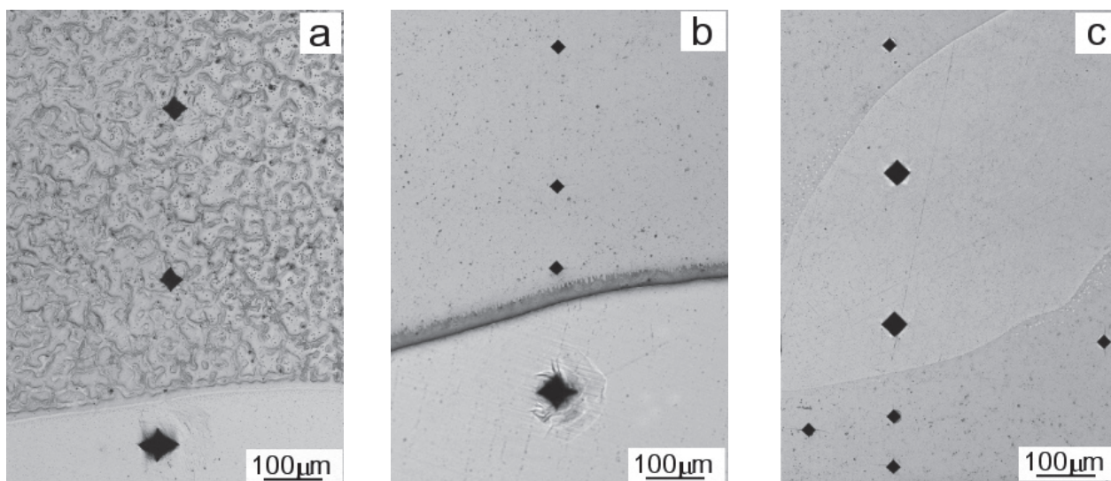
Fig. 6 Microhardness tester indentations in the Al-enriched layer and the Mg substrate: (a) layer fabricated at a higher current, (b) layer fabricated at a lower current, (c) traces of hardness measurements in \text{Al}_3\text{Mg}_2 phase and in area of solid solution Mg in Al
