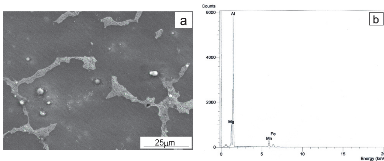
Fig. 4 (a) Distribution of white particles in the alloyed layer, (b) X-ray spectrum for a white particle
