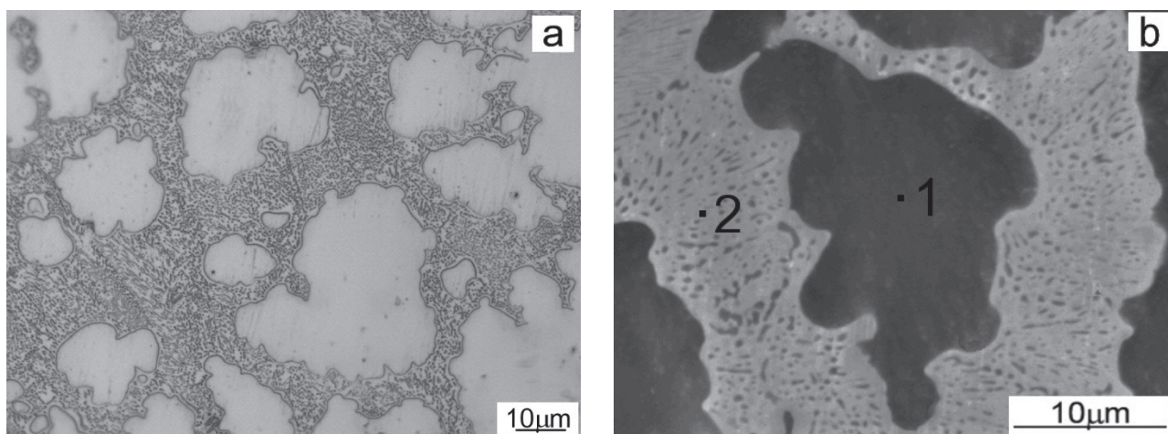
Fig. 3 Details of the layer microstructure observed at higher magnification: (a) OM image, (b) SEM image with the marked points of the EDS analysis
