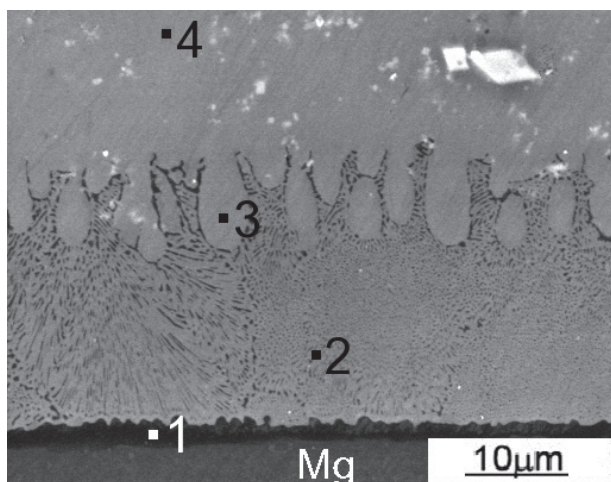
Fig. 5 SEM image showing details of the microstructure of the alloyed layer fabricated on Mg at a lower current with marked points of the quantitative EDS analysis.
