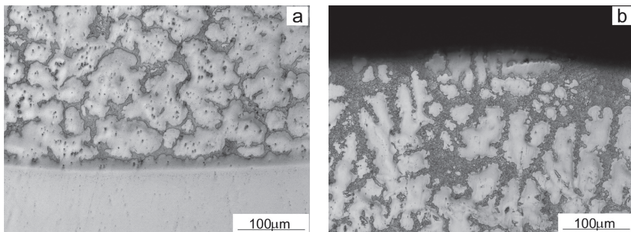
Fig. 2 Microstructure of the inner (a) and outer (b) zones in a layer fabricated on Mg at a higher current
