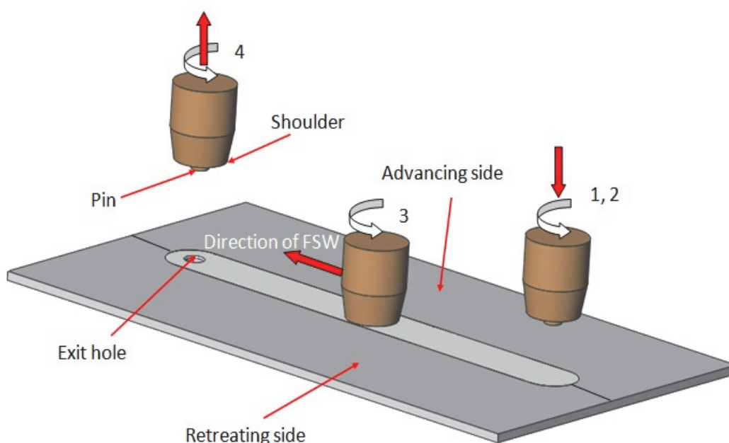
Fig. 1 Principal scheme of FSW
