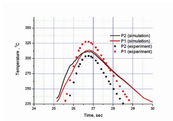
Fig. 6 Measured and calculated temperature during FSW (710 rpm, 400 mm/min of WS)
