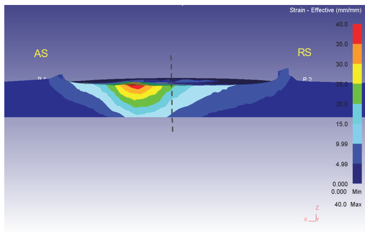
Fig. 5 Strain effective distribution (cross section view behind the pin)
