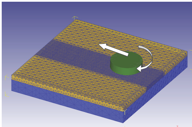
Fig. 2 FSW simulation model
