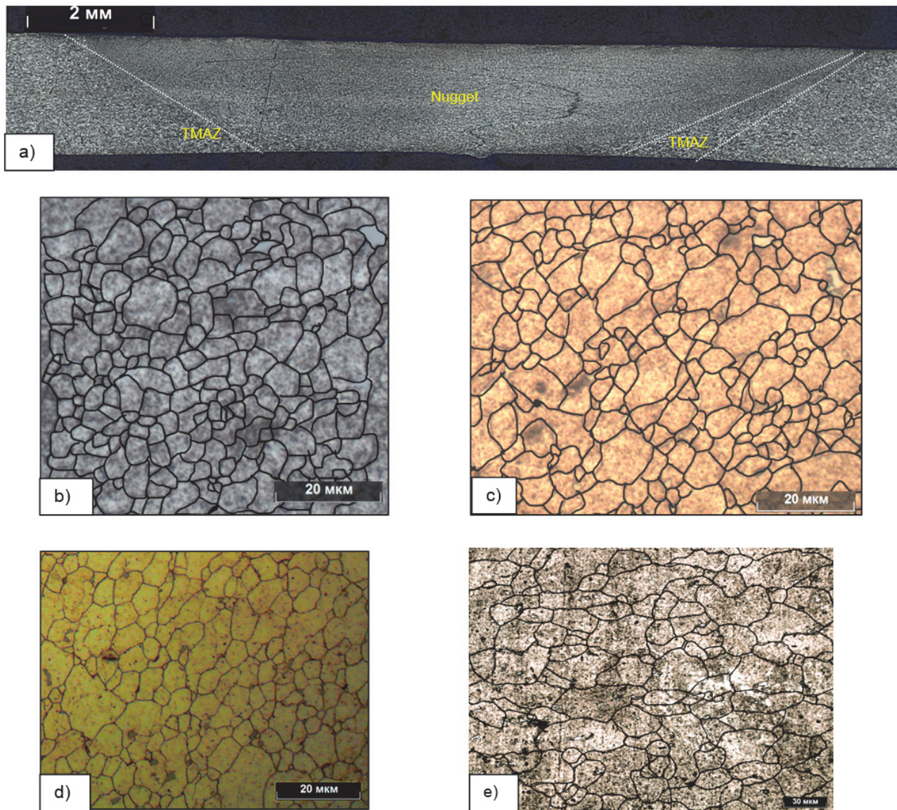
Fig. 7 FSW samples: a) Macrosample of FSWed sample with 710 rpm, WS of 400 mm/sec; b) Microstructure of FSW nugget (710 rpm); c) Microstructure of FSW nugget (900 rpm); d) Microstructure of FSW nugget (1120 rpm); e) Parent metal
