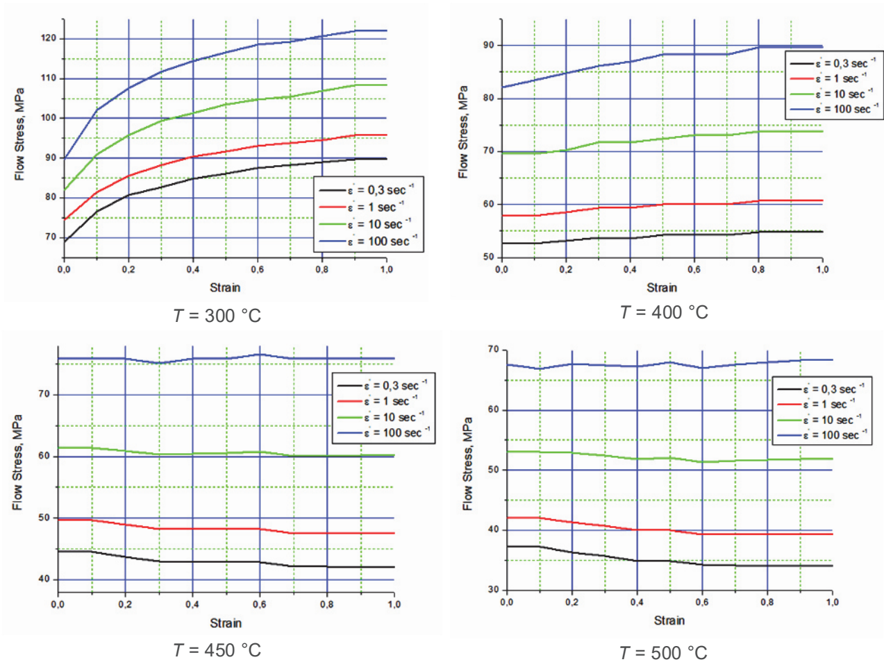
Fig. 3 Used rheology properties of Al 6082
