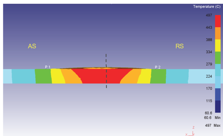
Fig. 4 Temperature field (cross section view)
