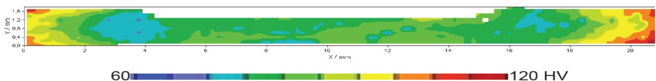
Fig. 8 Hardness test result (710 rpm, WS of 400 mm/min)
