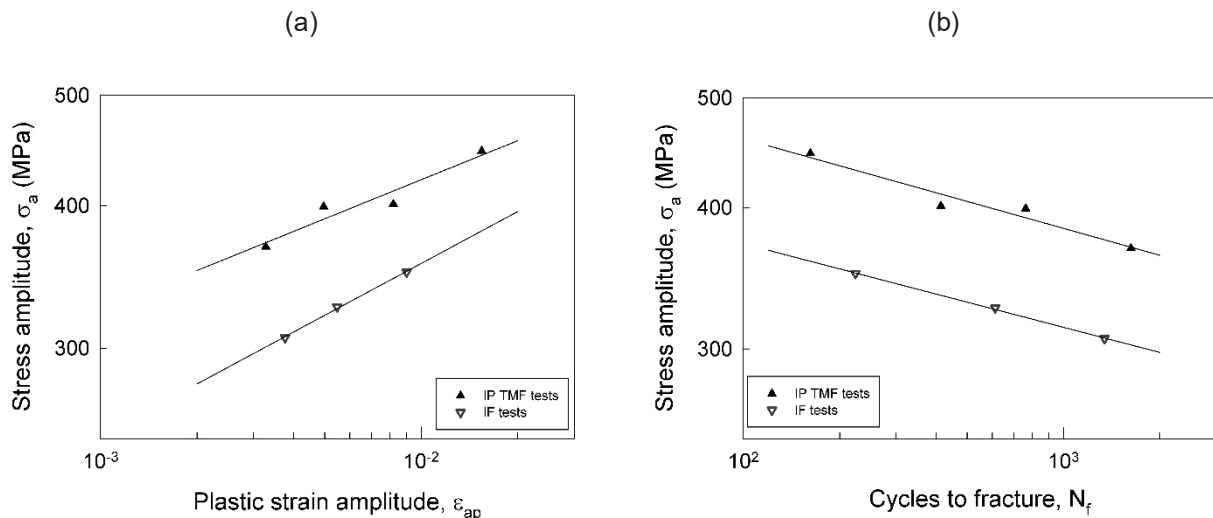
Fig. 3 Fatigue life curves for IP TMF and IF cycling (a) CSSCs and (b) Wöhler-Basquin
