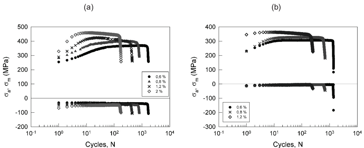
Fig. 2 Stress amplitude and mean stress vs. number of cycles, (a) IP TMF cycling, (b) IF cycling
