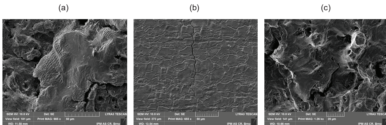
Fig. 4 (a) Transgranular cracking with striations under IF cycling, (b) and (c) mixed mode cracking under IP TMF cycling
