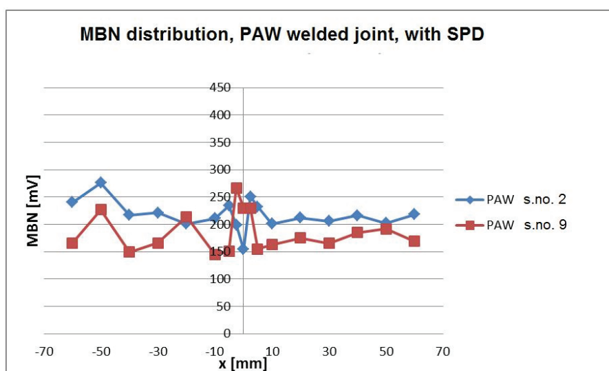
Fig. 10 Graph of the MBN distribution, six time DRECE, centre strip, sample no.2 and 9
