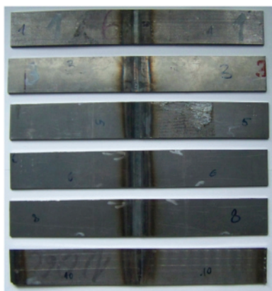
Fig. 11 Tensile test samples
