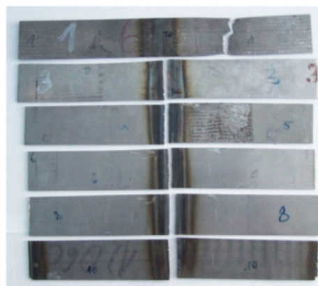
Fig. 12 Tensile test samples after fracture
