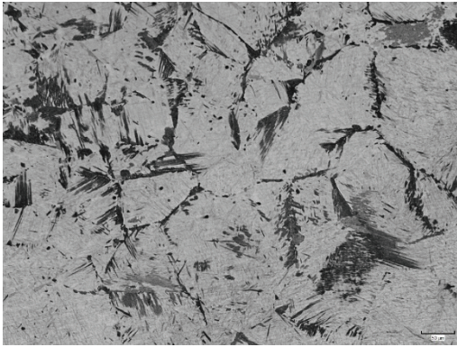
Fig. 3 Weld metal microstructure sample no.9, Nital etched
