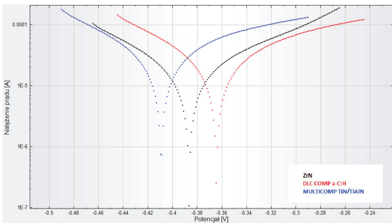
Fig. 4 The polarization curves in the 0.9% NaCl solution for the steel covered with ZrN, DLC COMP a-C:H and MULTICOMP TiN/TiAlN coatings
