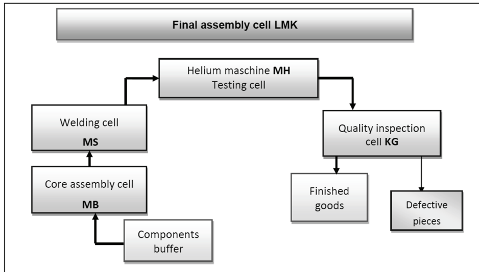
Figure 2 Final assembly cell LMK diagram
