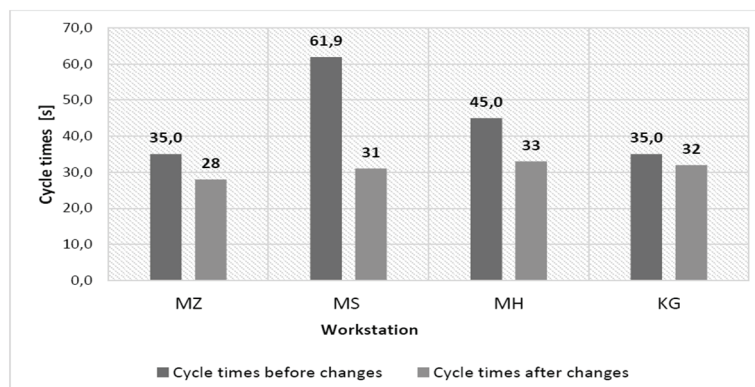
Figure 4 Analysis of cycle times in individual LMK cells
