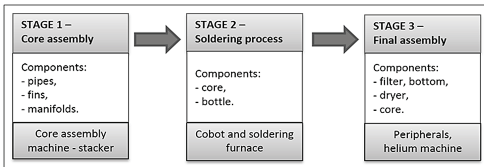
Figure 1 Production stages of the condenser
