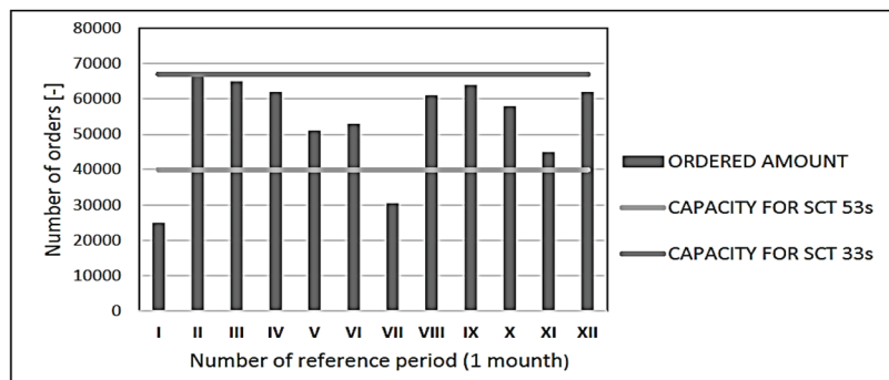
Figure 3 Comparison of orders with regard to line output
